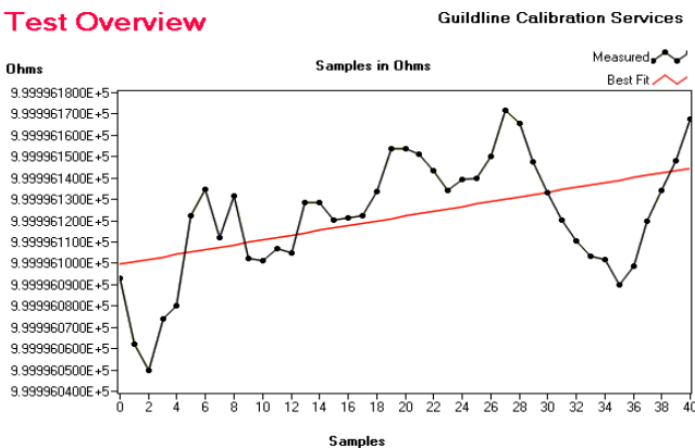
100:1 Transfer (10 kΩ to 1 MΩ)
